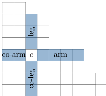
Figure 1.4: Limbs and co-limbs of a partition.
