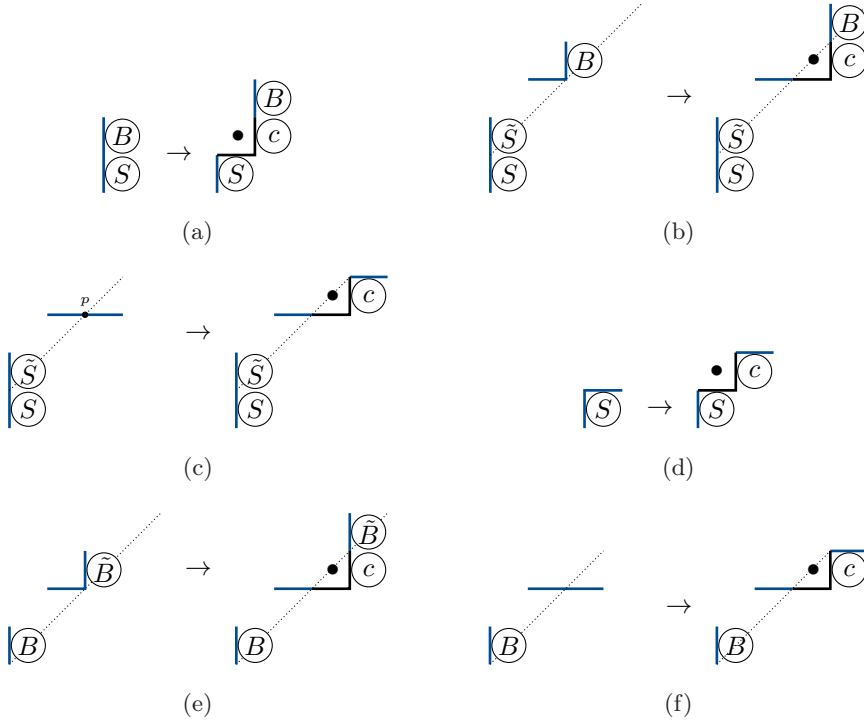
Figure 7.2: Surjectivity for i \geq s .
